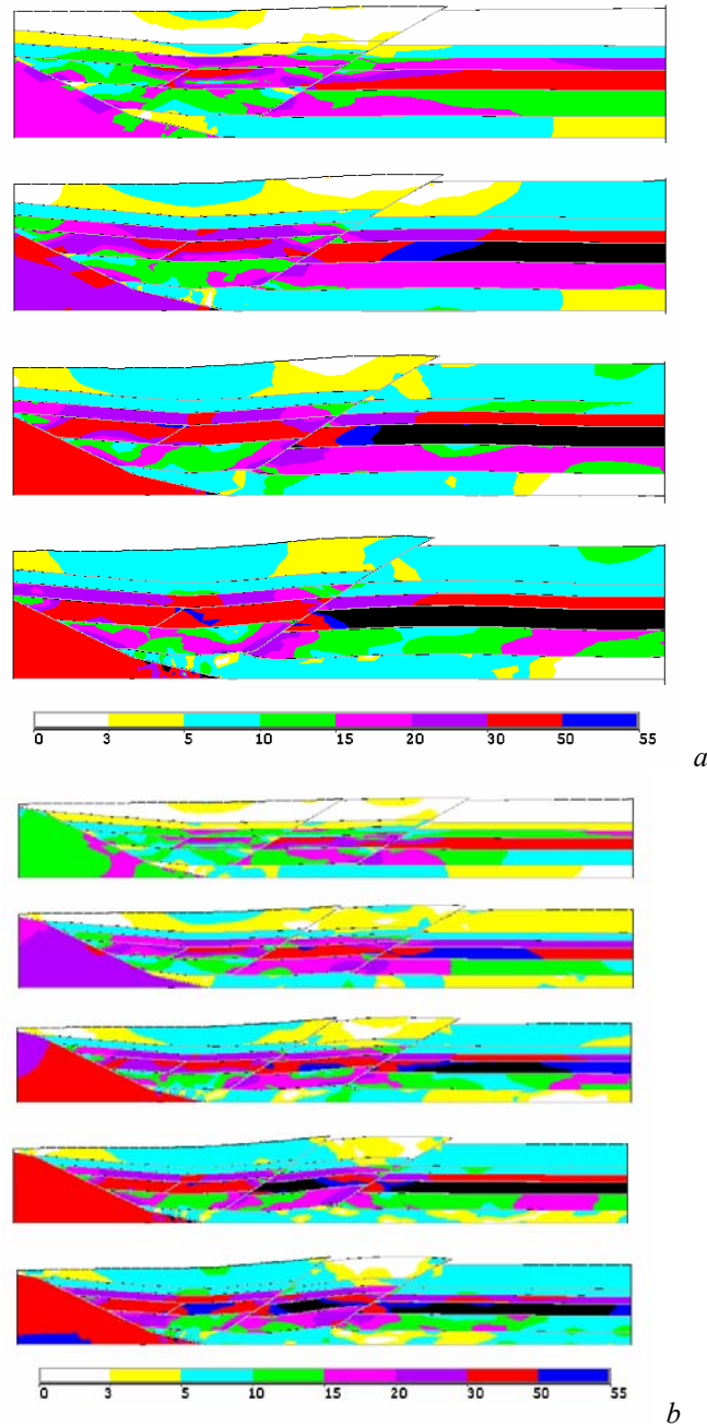
Fig. 2. Distributions of equivalent stresses \sigma_{eqv} (in MPa) for different stages during compression up to 2.5 km by step 0.5 km (top to bottom). Fragments of cross-section in the subduction zone are shown: a – model "6L-2F"; b – model "6L-3F" respectively.
